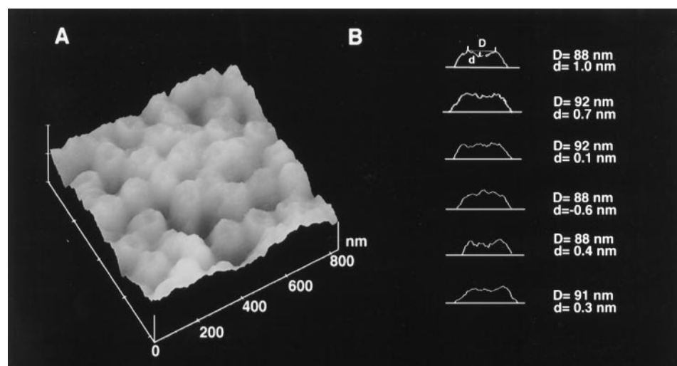
FIGURE 3 Images of NPCs in Ca 2+ -depleted solutions. (A) Nuclei were incubated in the low Ca 2+ (free Ca 2+ \sim 5 nM) and imaged over an \sim 4 \mu\text{m}^2 area. (B) Sample profiles of Ca 2+ -depleted NPCs showing the range of measurements. Distances d and D are the same as defined in Fig. 2.
