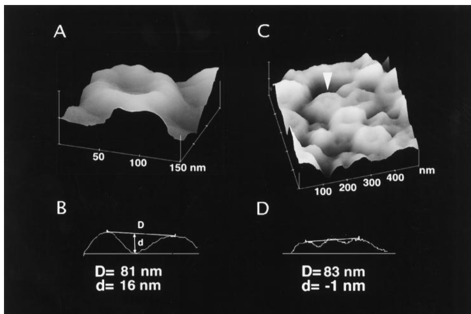
FIGURE 2 Three-dimensional images of Xenopus oocyte NPCs in MIB solution. (A) Image of one NPC incubated in normal ( 200 \text{ nM} free [\text{Ca}^{2+}] ) \text{Ca}^{2+} -containing medium. The AFM imaged NPC has the characteristic eightfold symmetry described in previous 2D electron microscopy. (B) Profile of the NPC showing an unusually recessed central depression ( \sim 16 \text{ nm} in depth ( d ) as measured from the midpoint between the peaks of the NPC outer vestibule ( D = 81 \text{ nm} ) to the lowest point between peaks). (C) Image of NPCs in which the central granule has shifted to occlude the central depression by \text{Ca}^{2+} depletion. (D) NPC profiles of (C) revealing occlusion of the central depression ( d = -1 \text{ nm} indicates that the central granule is 1 \text{ nm} above the surrounding cytoplasmic rings).
